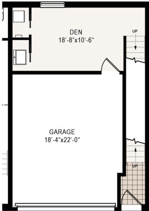
-1 GROUND FLOOR PLAN NOT TO SCALE
